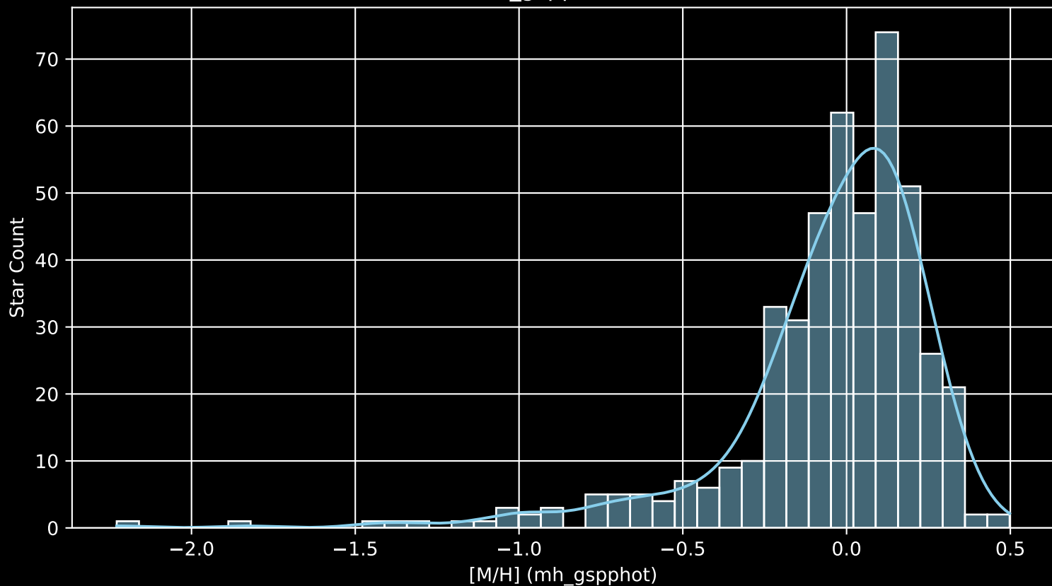
APOGEE DR17 Field: [340-06 [M/H] (mh_gspphot) (n= 462)
