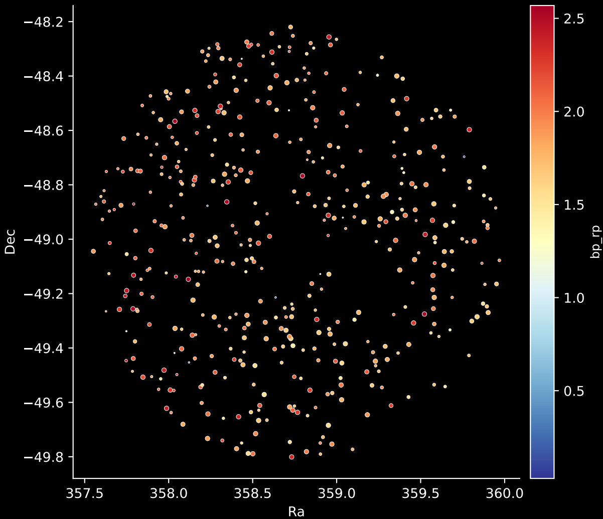
APOGEE DR17 Field: [340-06] Stars: 464
