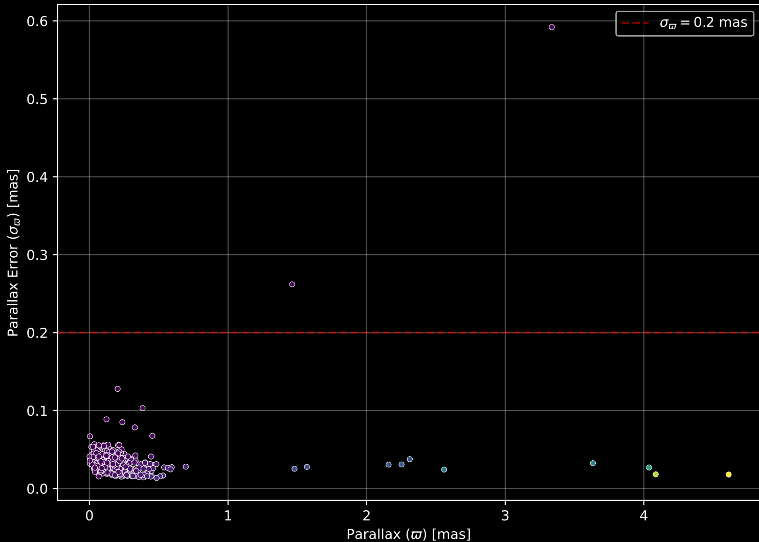
APOGEE DR17 Field: [340-06] Parallax Quality (n= 464)
