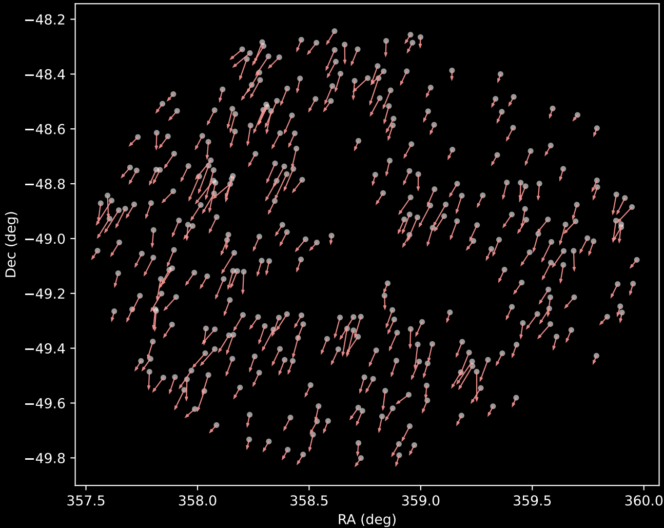
APOGEE DR17 Cluster 7 Proper Motion Vectors (n=322)
