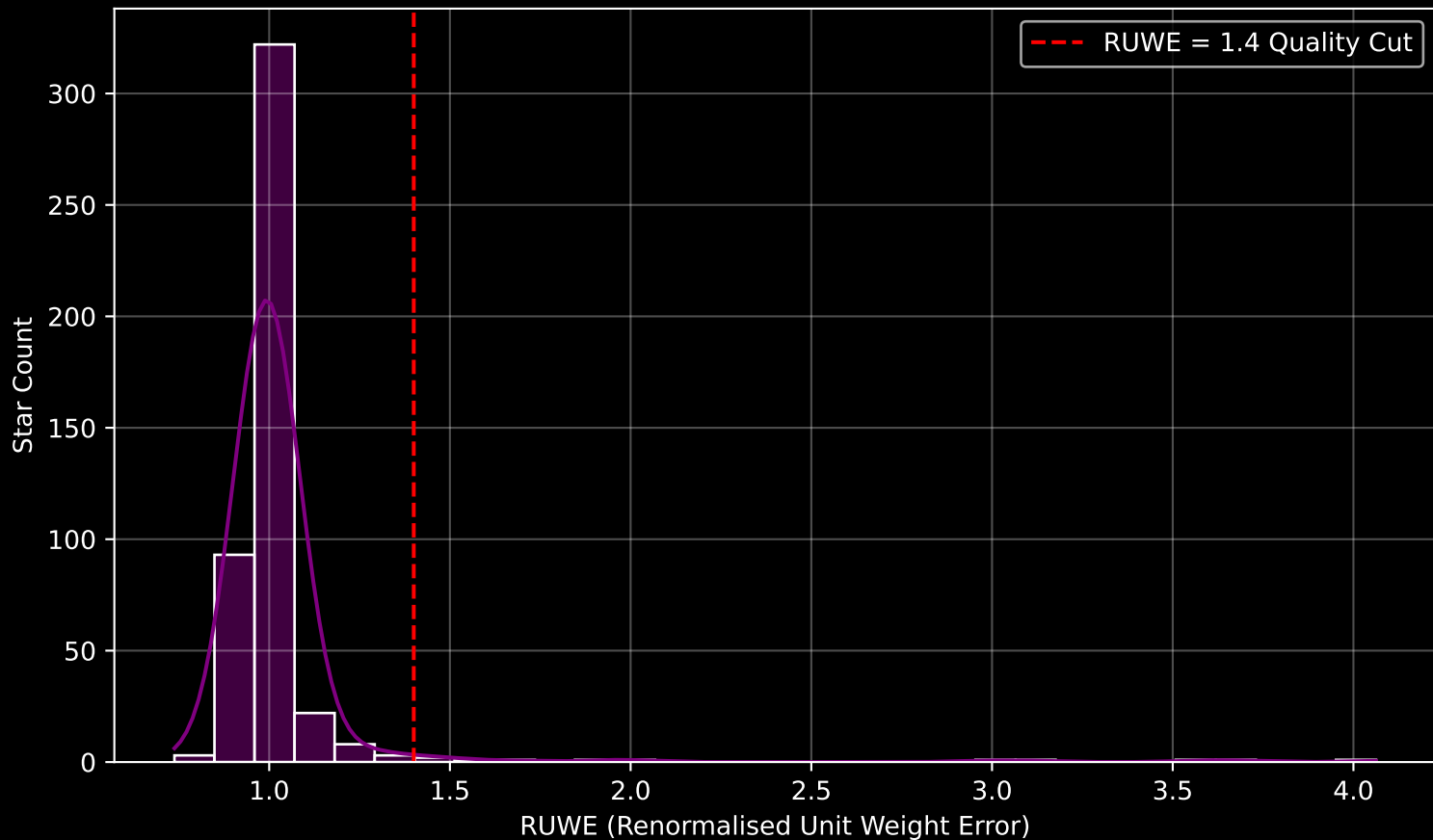
GAPOGEE DR17 Field [340-06] RUWE Distribution (n= 462)
