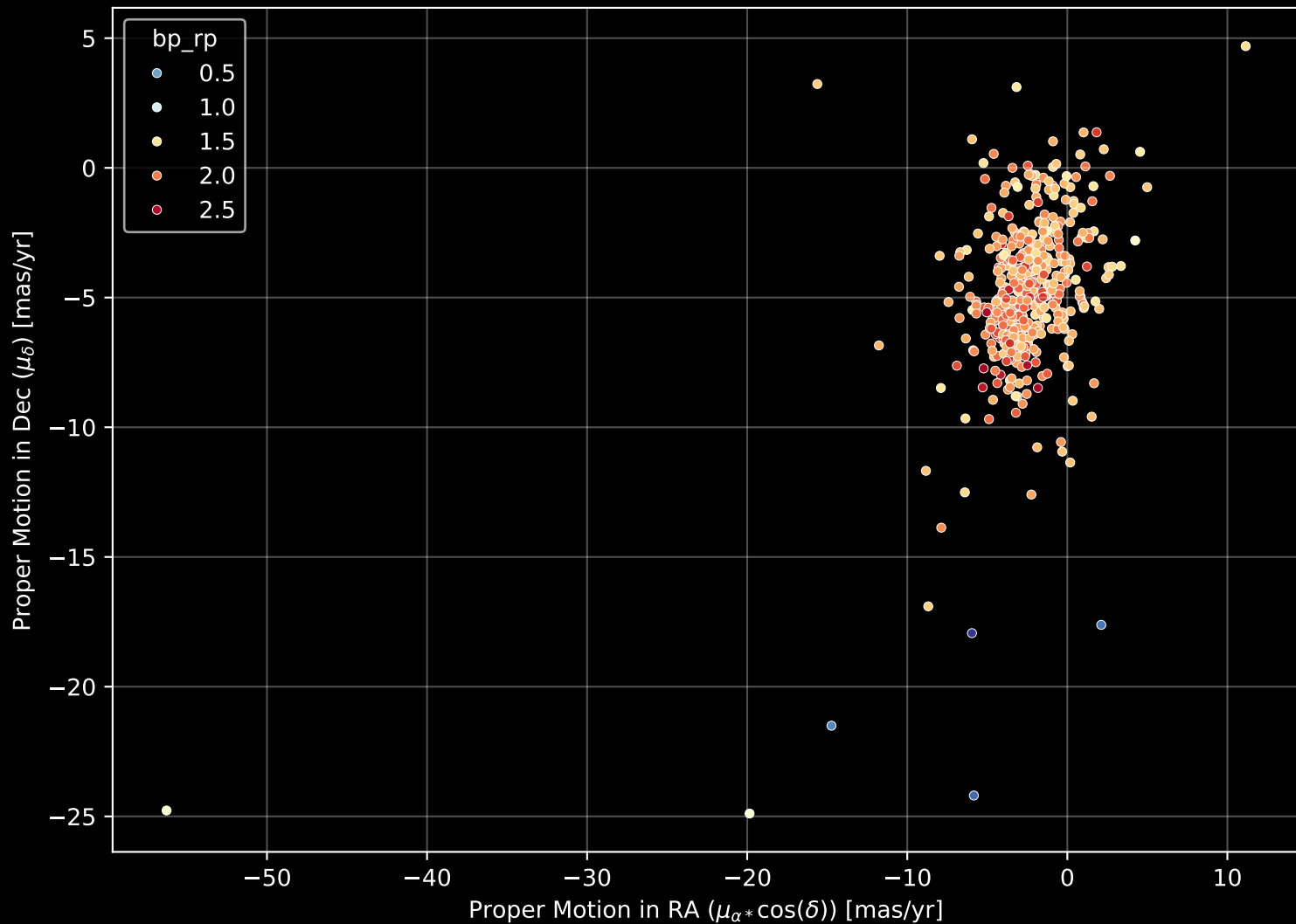
APOGEE DR17 Field: [340-06] Proper Motion Diagram (n= 464)
